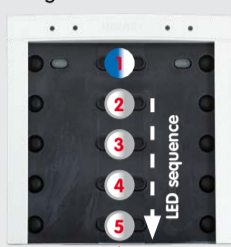
Pattern 1 (MX-Bell-Button-F1): LED 1 permanently blue (function button) LEDs 2 to 5 flashing white 4 (bell buttons)
